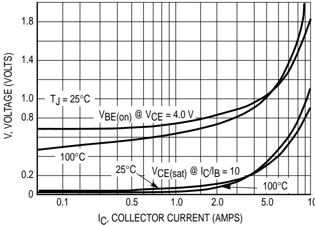
Figure 5. "On" Voltages
