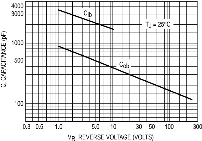
Figure 2. Capacitances
