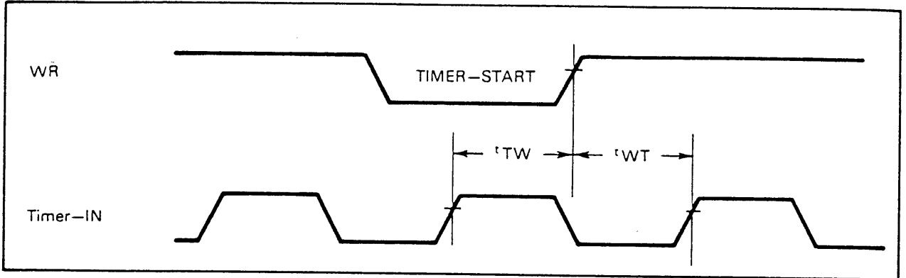
Timer Waveforms 2
