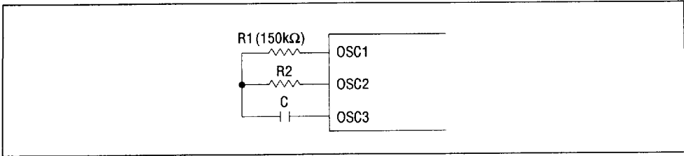
Figure 11 RC Oscillation Connection Circuit
