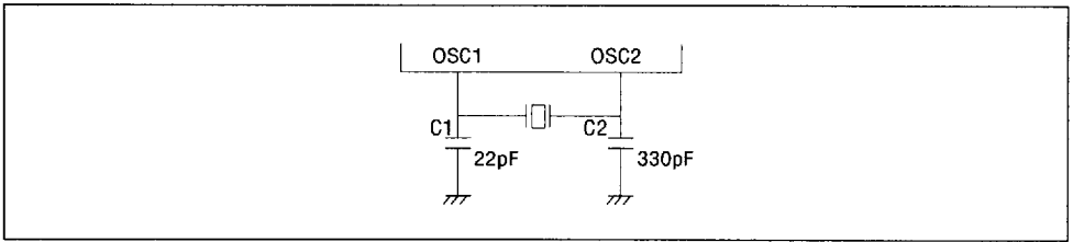
Figure 13 Circuit Diagram of Crystal Oscillator Connection
