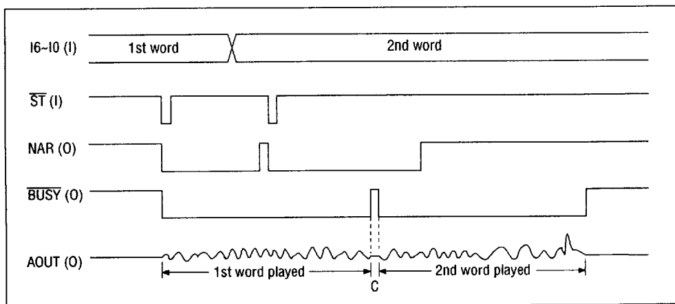
Figure 1 Timing of CPU Interface ( \overline{ST} \leq 350 \mu S )
