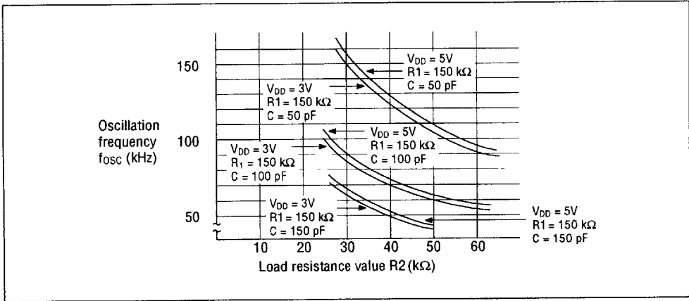
Figure 12 RC Oscillation Frequency Characteristics
