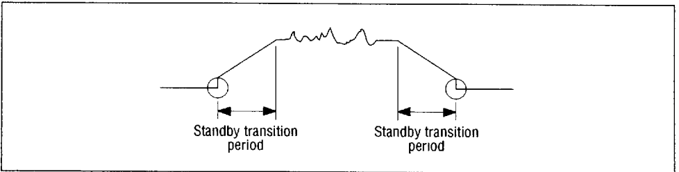
Figure 9 Pop Noise of Low-pass Filter Output
