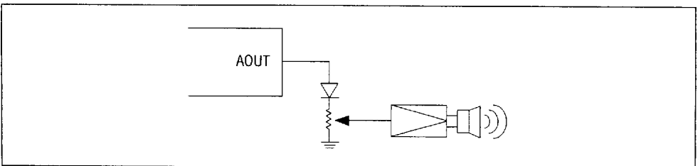
Figure 10 Pop Noise Suppression Circuit
