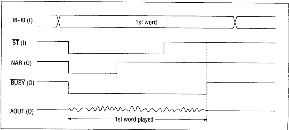
Figure 3 Timing of SW Input Interface (playing one word)
