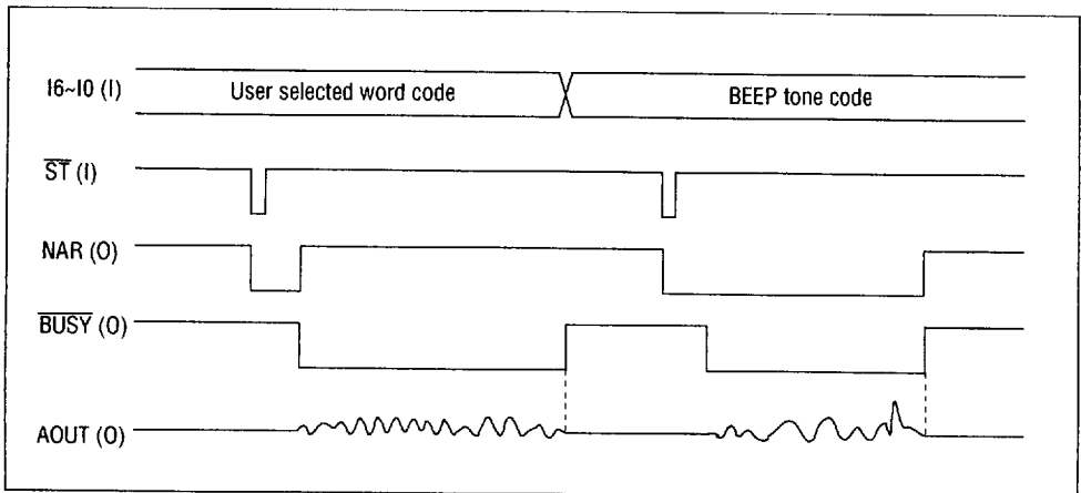
Figure 5 Timing at BEEP Tone Generation
