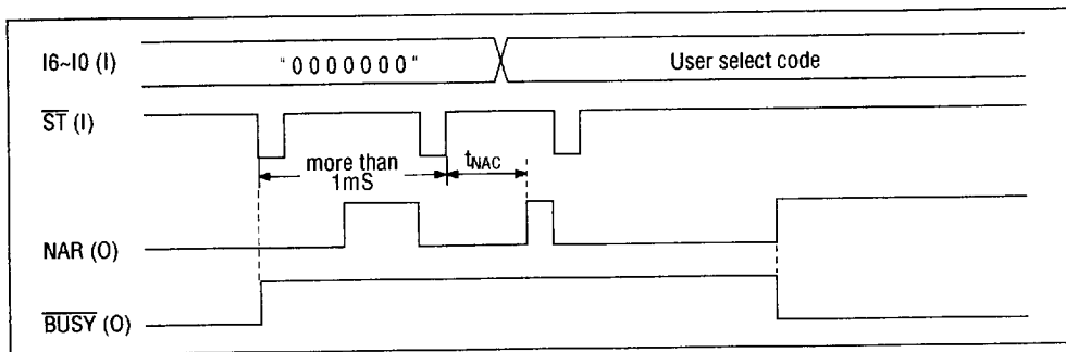
Figure 6 Example of STOP Code Input Timing
