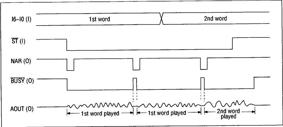
Figure 4 Timing of SW Input Interface (repeated play)
