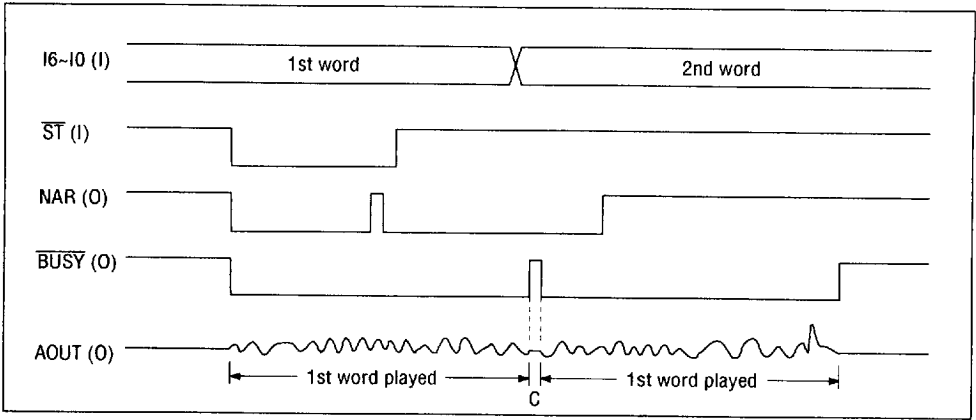
Figure 2 Timing of CPU Interface ( \overline{ST} > 800 \mu\text{S} )
