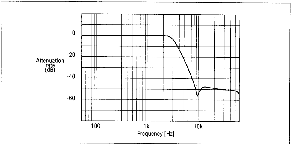
Figure 8 Low-pass Filter Characteristics ( f_s=8 kHz)
