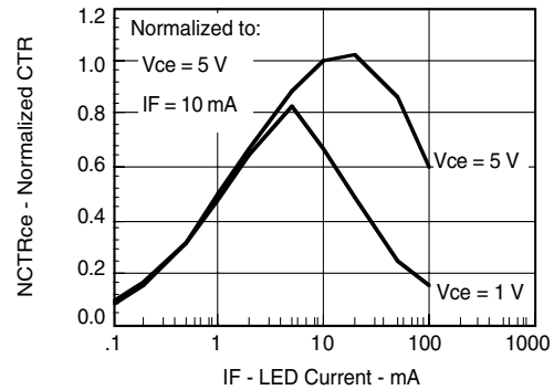
Fig. 2 Normalized Non-Saturated and Saturated CTR vs. LED Current
