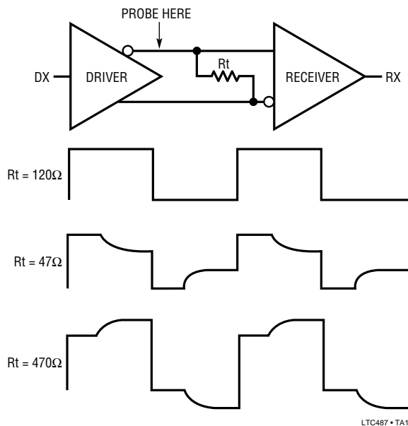
Figure 9. Termination Effects
