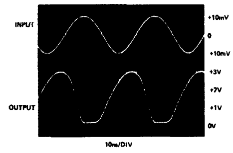
RESPONSE TO 25MHz SINE WAVE
