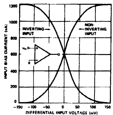
INPUT BIAS CURRENT vs DIFFERENTIAL INPUT VOLTAGE
