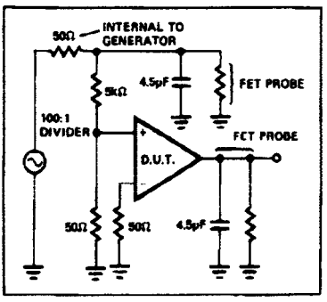
RESPONSE PHOTOGRAPH TEST SET-UP
