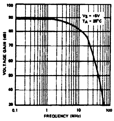
VOLTAGE GAIN vs FREQUENCY
